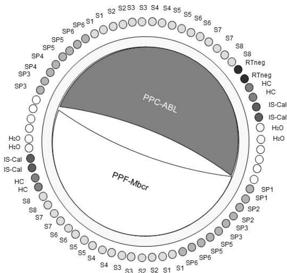
Figure 4. Suggested rotor setup for each experiment with the ipsogen BCR-ABL1 MbcR IS-MMR DX Kit. SP1–SP6: BCR-ABL MbcR and ABL standards; HC: High cDNA positive control; IS-Cal: IS-MMR calibrator; RTneg: RT negative control; S: cDNA sample; H 2 O: water control.
