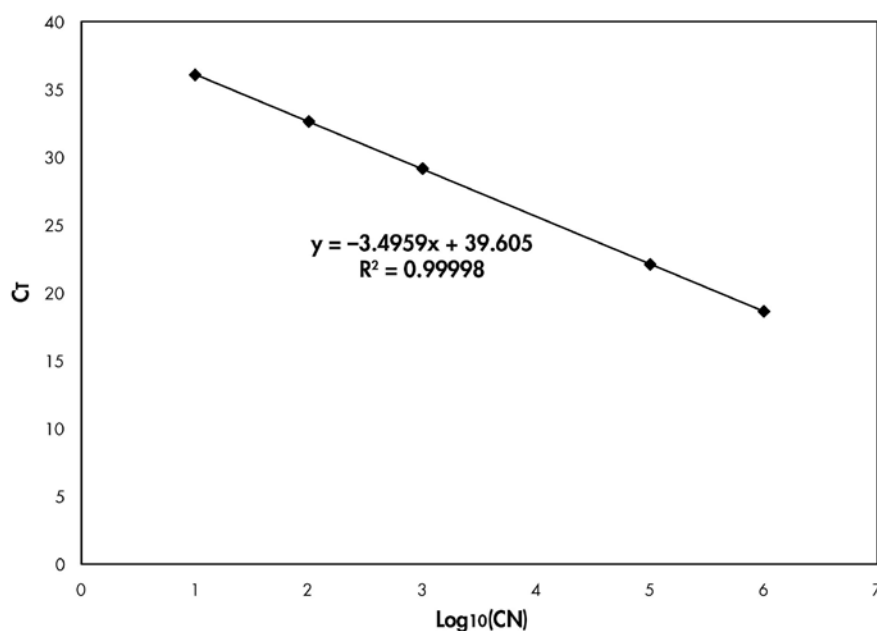
Figure 10. Theoretical curve for BCR-ABL calculated from 5 standard dilutions. A linear regression curve ( y = ax + b ) is calculated, where a is the slope of the line and b is the y -intercept, which is the y -coordinate of the point where the line crosses the y axis. Its equation and coefficient of determination ( R^2 ) are printed on the graph.
