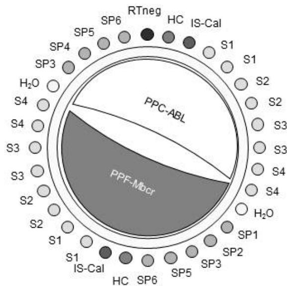
Figure 6. Suggested rotor setup for each experiment with the ipsogen BCR-ABL1 Mbcr IS-MMR DX Kit. SP1–SP6: BCR-ABL Mbcr and ABL standards; HC: High cDNA positive control; IS-Cal: IS-MMR calibrator; RTneg: RT negative control; S: cDNA sample; H 2 O: water control.
