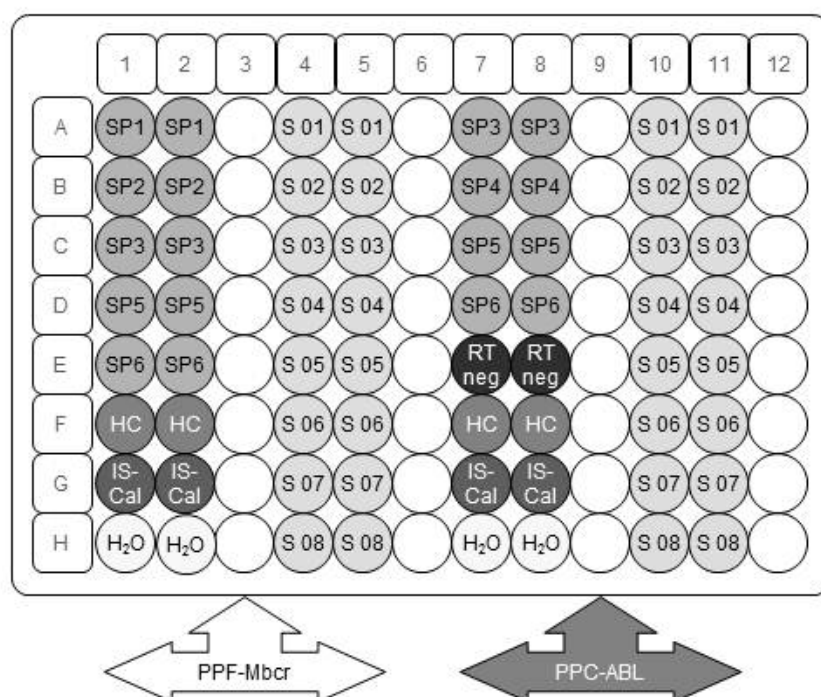
Figure 5. Suggested plate setup for one experiment with the ipsogen BCR-ABL1 MbcR IS-MMR DX Kit. SP1–SP6: BCR-ABL MbcR and ABL standards; HC: High cDNA positive control; IS-Cal: IS-MMR calibrator; RTneg: RT negative control; S: cDNA sample; H 2 O: water control.
