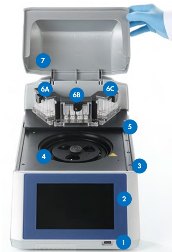
1. PyroMark Q48 Autoprep instrument front, open view.
