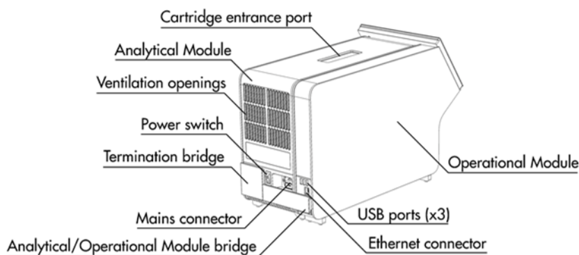
Figure 2. Rear view of QIAstat-Dx Analyzer 2.0. The Operational Module is on the right and the Analytical Module is on the left.
